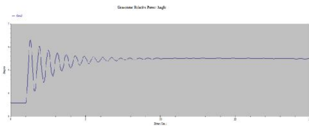
Figure 4.13 Swing curve of the generator
