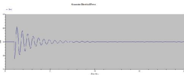
Figure 4.14 Real power P of the Generator
