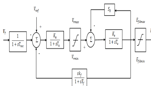
Figure 2.2 Block diagram of type 1 AVR
