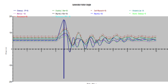
Figure 3.4 Swing curves of the generators for changing the droop constant
