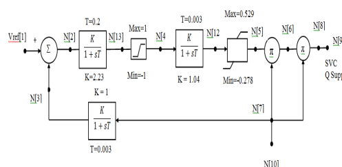
Figure 2.1. Modeling of SVC
