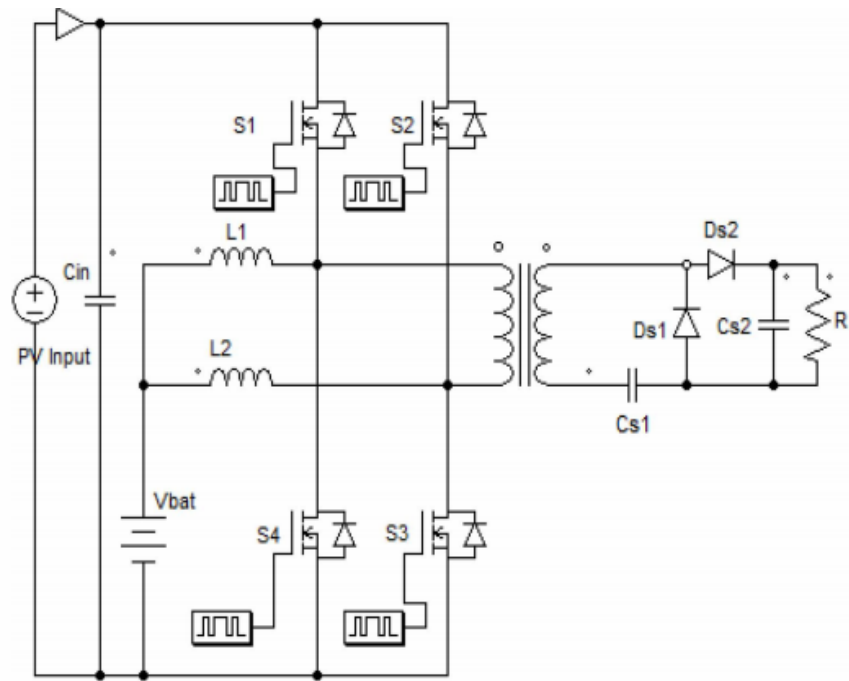
Figure 1: Two-port Converter with Output Voltage Doubler
