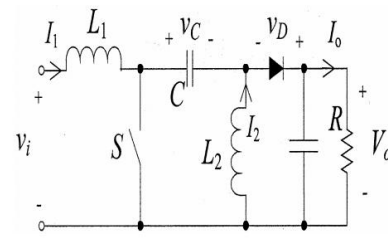
Figure 7: SEPIC Converter
