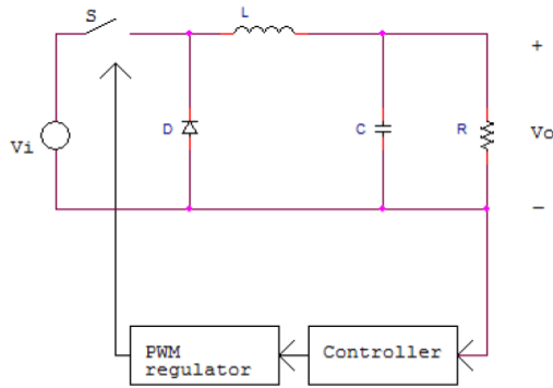
Figure 3: Buck Converter
