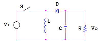
Figure 5: Buck-boost Converter
