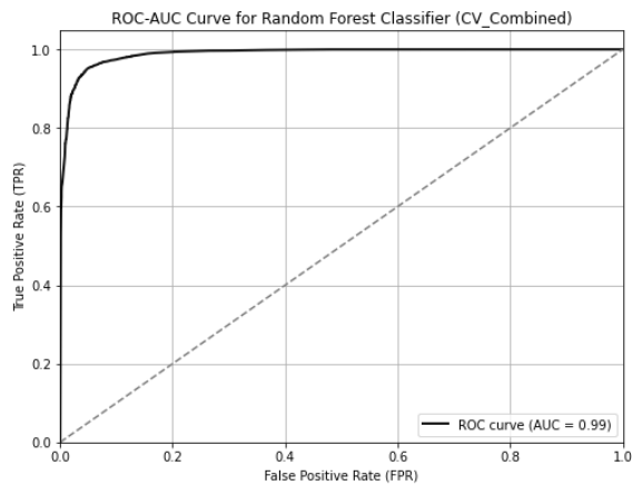
Figure 1. ROC-AUC curve for Count Vectorizer
