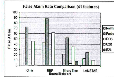
Fig. 4 False Alarm Rate Comparison (41 features)
