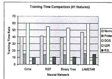
Fig. 6 Training Time Comparison (41 features)
