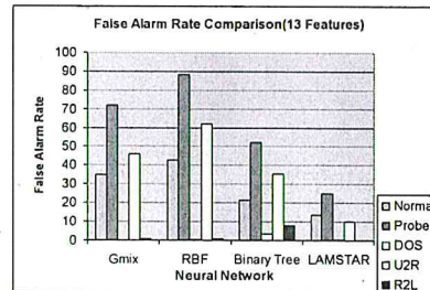
Fig. 5 False Alarm Rate Comparison (13 features)
