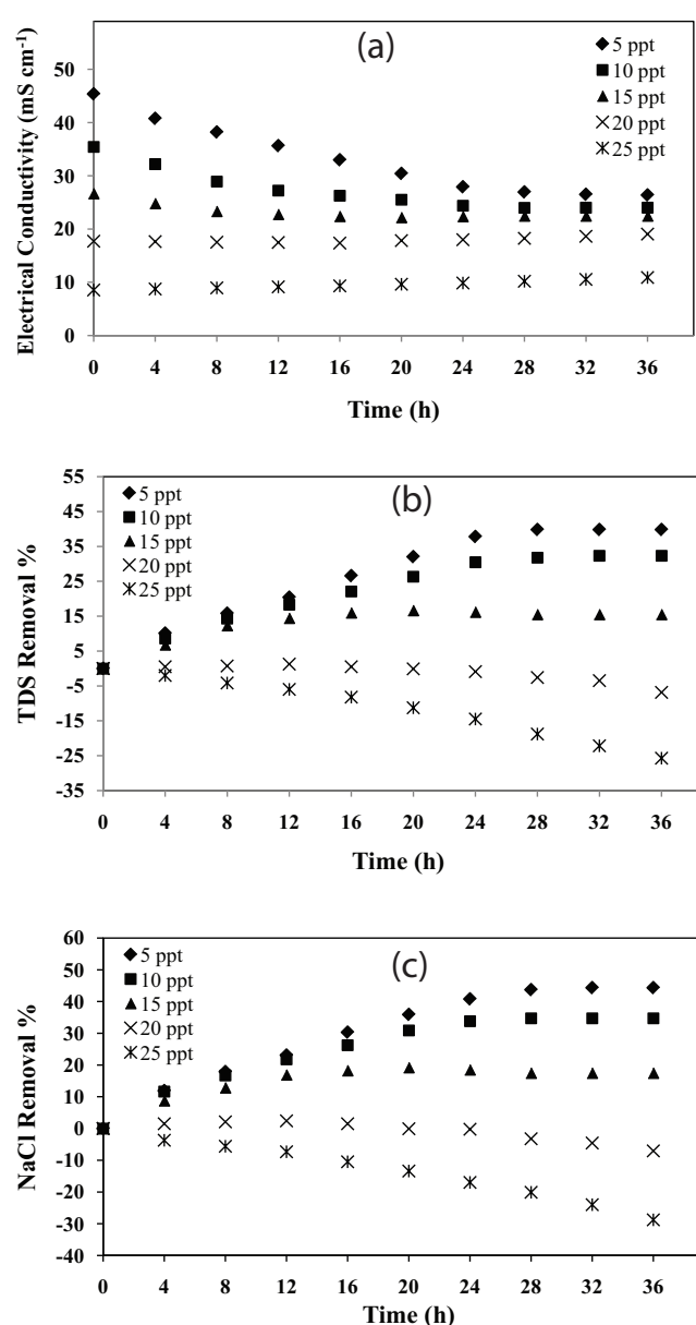
Fig. 4. (a) Electrical conductivity change, (b) TDS removal percentage, and (c) NaCl removal percentage for 15% algae ratio at different TDS concentrations.
