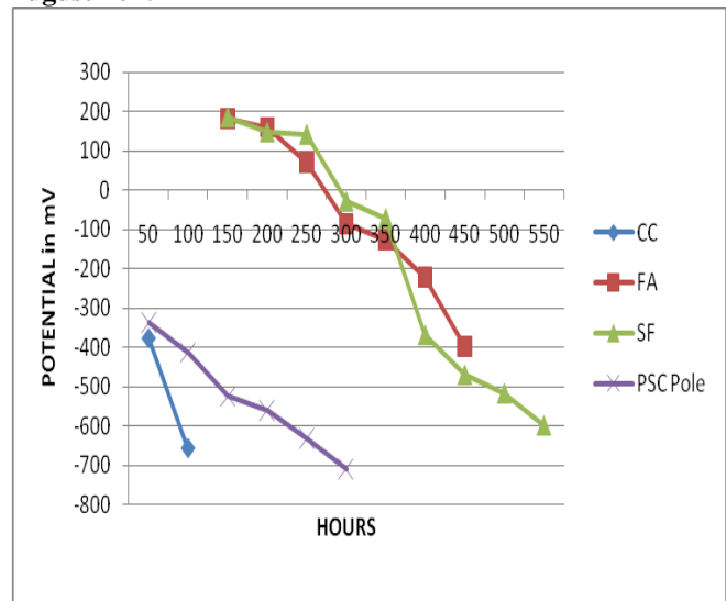
Fig.5 Corrosion exposure for conventional concrete Vs Different mixes
