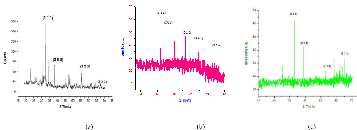
Fig. 1 XRD spectrum of (a) undoped CdO films (b) 4% Cu doped CdO thin films (c) 8% Cu doped CdO thin films
