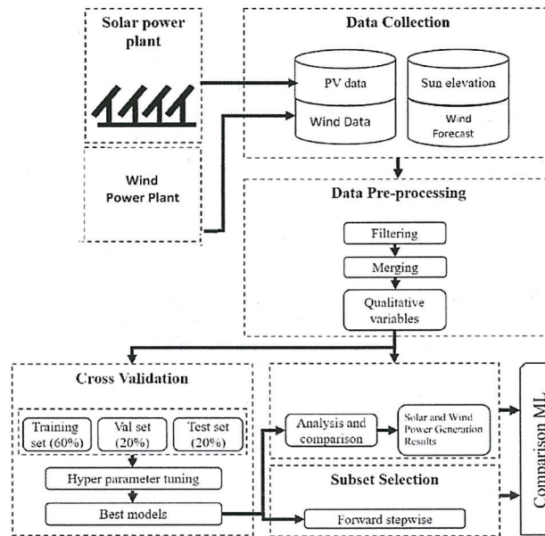
Figure 6. Application of machine learning in renewable energy prediction
