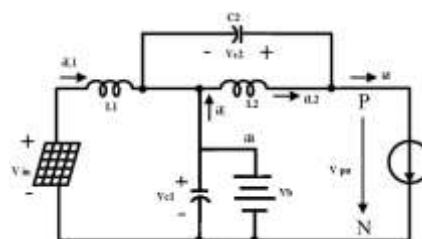
Fig 3.3 mode 2 operation
