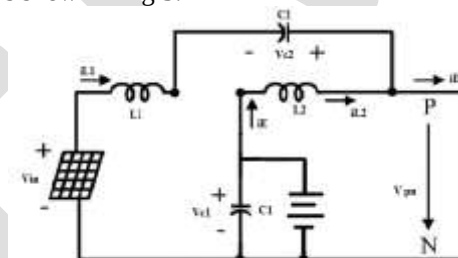
Fig 3.2 Mode 1 operation
