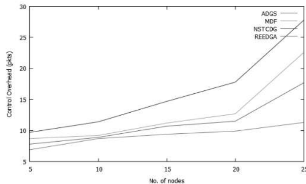
Fig. 8 : Control Overhead Vs No. of Nodes
