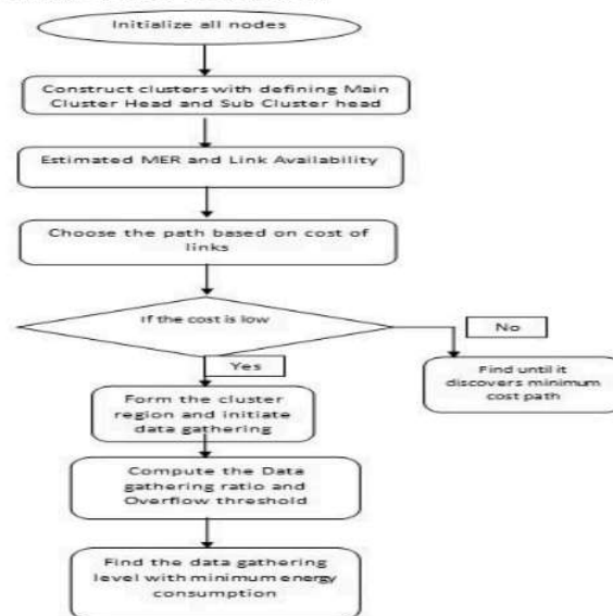
Fig. 1: Flow of Proposed Data Gathering Approach
