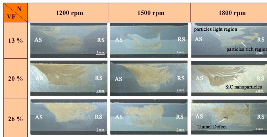
Fig. 3 – Cross-sectional structures of Lap-FSW joints at different weld condition.
