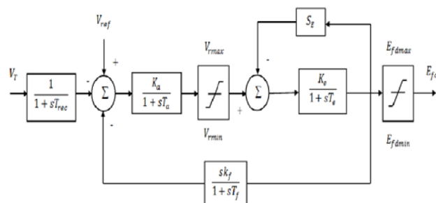
Fig. 2.2 Block diagram of type 1 AVR
