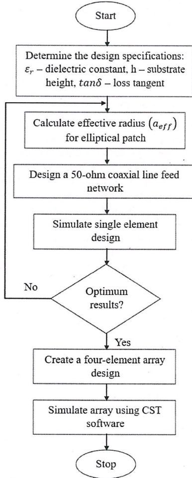
Fig. 1. Microstrip patch array antenna design flowchart.
