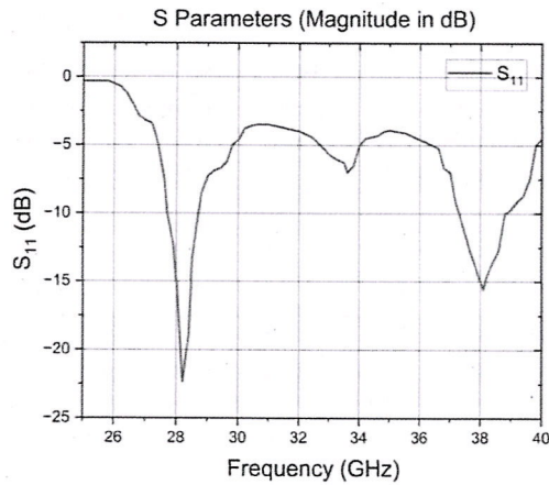
Fig. 4. Return loss for a 38 GHz and 28 GHz patch antenna array.
