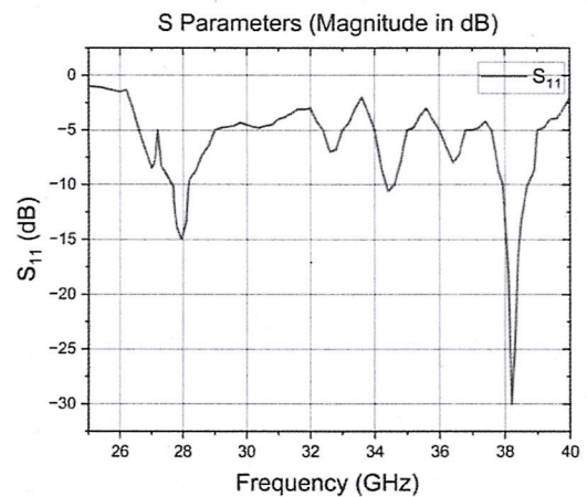
Fig. 6. Antenna array for an SIW return loss.
