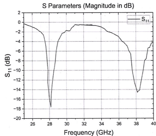
Fig. 3. Return loss for a single-element patch antenna.
