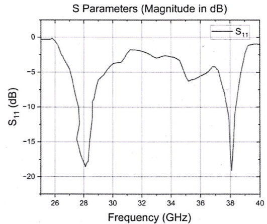
Fig. 5. Return loss for a single slotted in-plane element.
